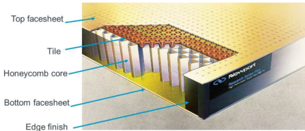
Figure 2. Structure of the optical breadboard. Adapted from MKS Instruments 1 .
