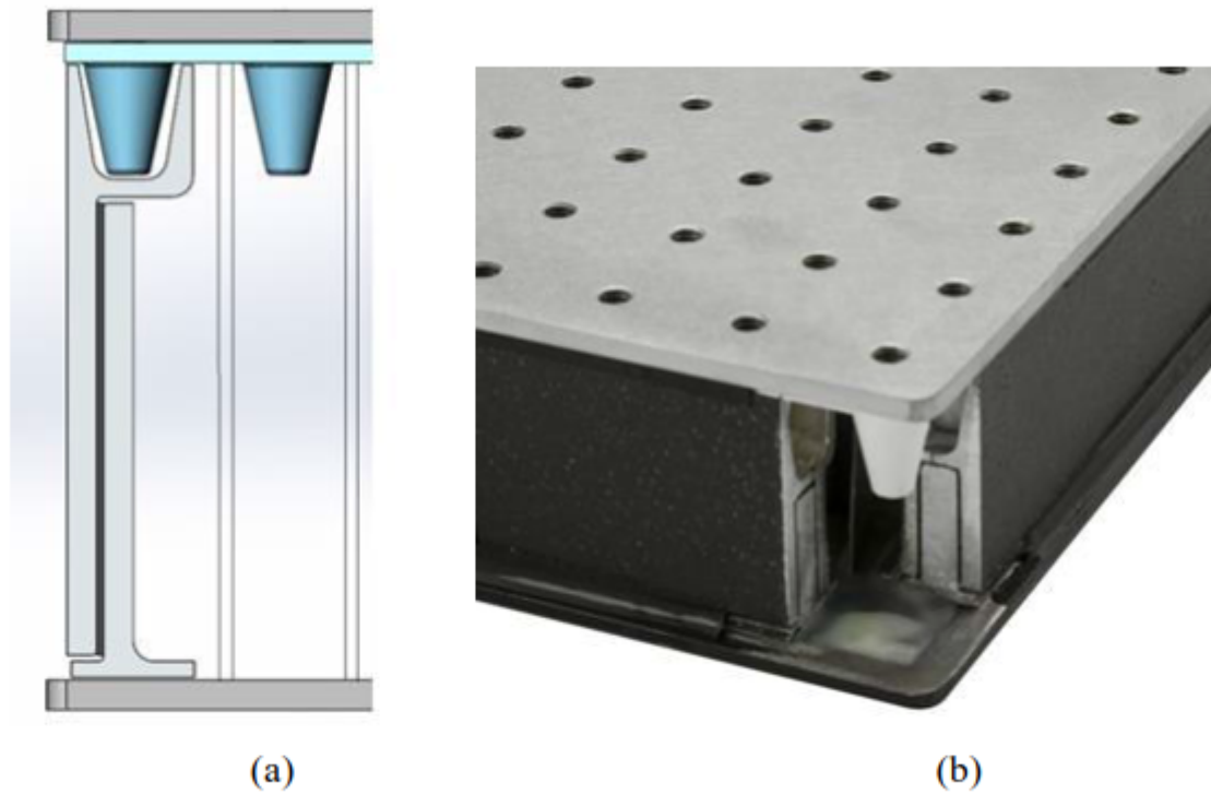
Figure 13. (a) Sketch design of the damped edge finish for the 110 mm breadboard; (b) Photo of a 59 mm breadboard with damped edge finish (corner piece removed for sake of illustration), adapted from MKS Instruments 1 .
